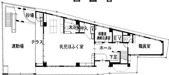
(1F)
